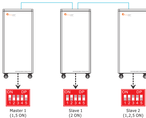
Example of three batteries in parallel
